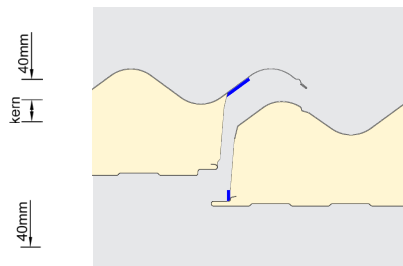
detail montage
